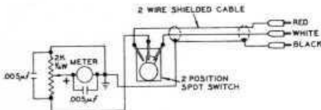
SCHEMATIC DIAGRAM, DIRECTIONAL COUPLER INDICATOR FIGURE 2.
