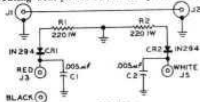
FIGURE 1 DIRECTIONAL COUPLER SCHEMATIC
