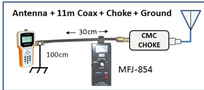
ANT TEST 4 Config. 1D
