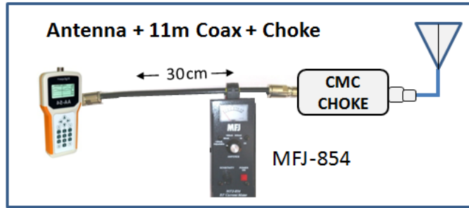
ANT TEST 3 Config. 1C
