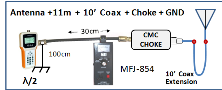
ANT TEST 8 Config. 2D
