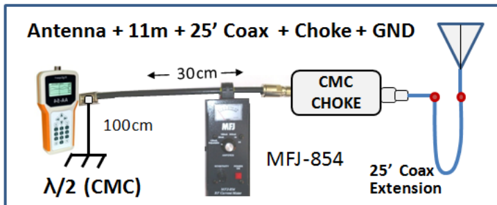
ANT TEST 12 Config. 3D
